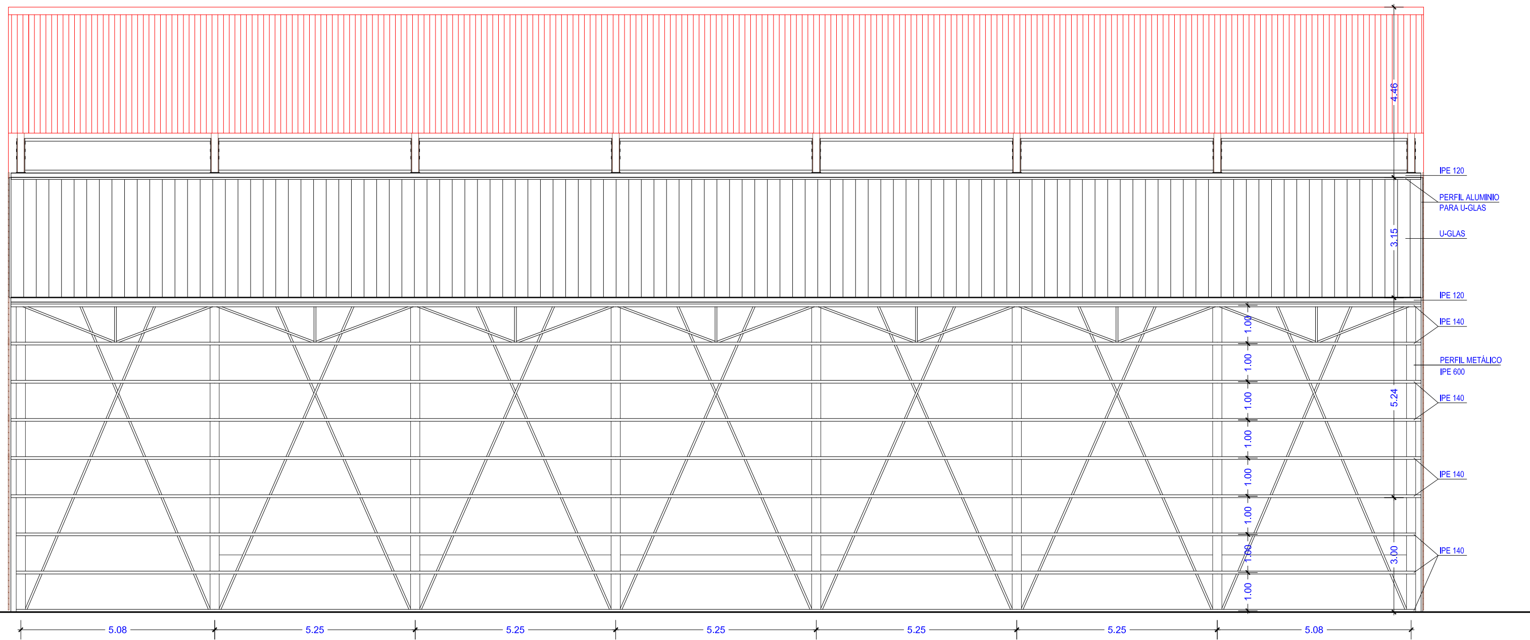
FACHADA PRINCIPAL
